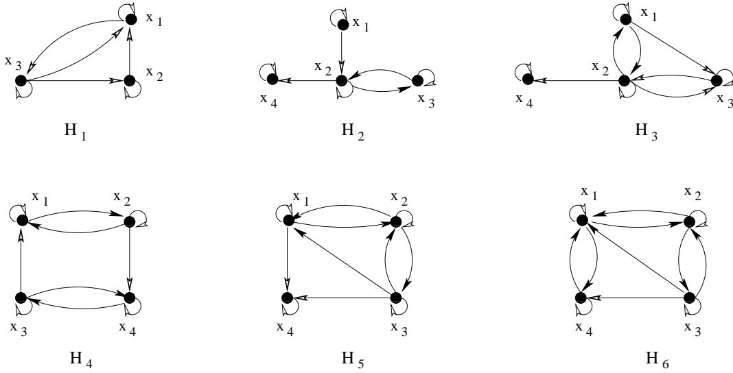
Figure 1: The obstructions H_i with i = 1, 2, 3, 4, 5, 6 .
