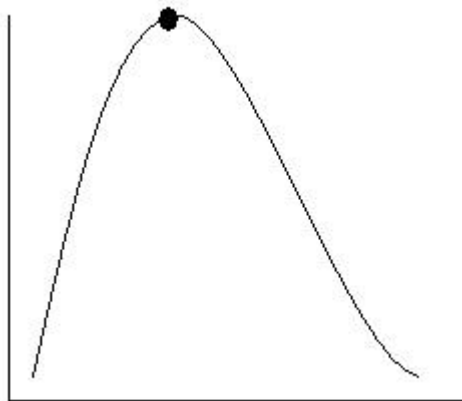
Figure 5.1. EM converges to global maximum in Model 1
