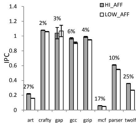
Figure 5. IPC on MMP
