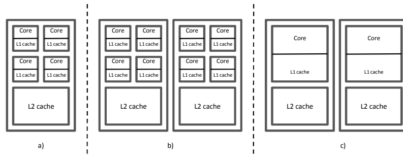
Figure 1. Schematic view of (a) a multicore uniprocessor consisting of a single chip and four cores, (b) multicore multiprocessor consisting of two multicore chips, and (c) a conventional multiprocessor consisting of two uniprocessor chips.
