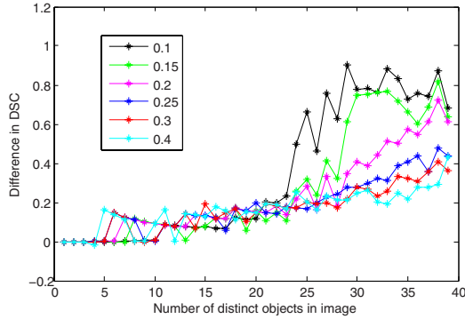
Fig. 7. (Color figure, refer to e-copy). Difference in average DSC between adaptive regularization GC and standard GC for images with increasing numbers of ellipses. Different curves represent different noise standard deviations as shown in legend. Positive DSC difference indicates adaptive regularization GC is more successful than standard GC at labeling ellipses with low image quality.
