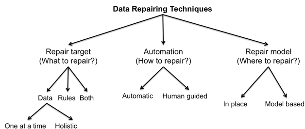
Figure 2: Classification of data repairing techniques.
