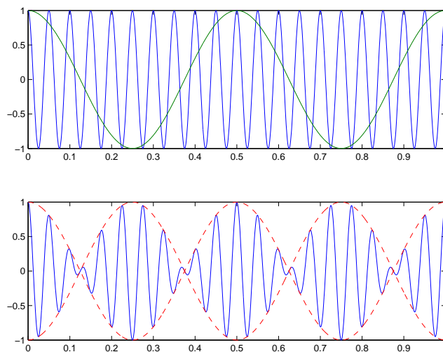
Figure 3: An example of amplitude modulation.
