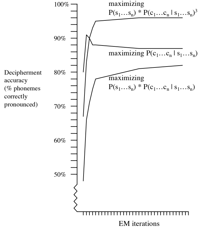
Figure 5: Performance of Spanish decipherment. As we increase the number of EM iterations, we see an improvement in decipherment performance (measured in terms of correctly generated phonemes). The best result is obtained by weighting the learned spelling model more highly than the sound model, i.e., by choosing a phonetic decoding s_1 \dots s_n for character sequence c_1 \dots c_n that maximizes P(s_1 \dots s_n) \cdot P(c_1 \dots c_n | s_1 \dots s_n)^3 .
