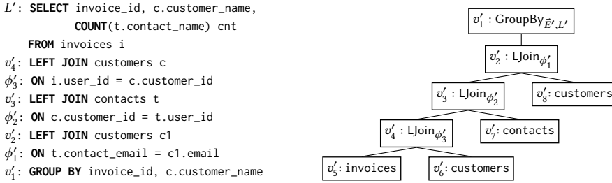
Fig. 2. SQL query P' (left) and its corresponding AST (right), following the same protocol as in Figure 1.
